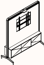
Digital-03 Digital Display & Joinery OW 1690mm OD 650mm OH 1950mm
