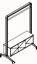
Storage-04 Hanging rail & Joinery OW 1290m OD 650mm OH 1950mm
