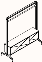
Storage-04 Hanging rail & Joinery OW 1690mm OD 650mm OH 1950mm
